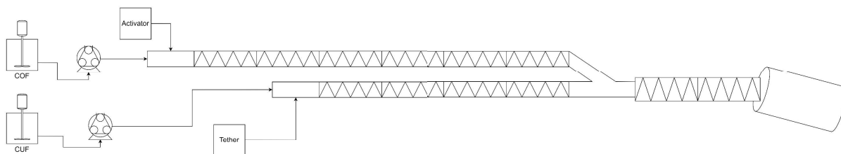
Figure 4 Schematic of static mixer rig
