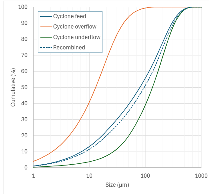
Figure 2 Particle size distribution of tailings
