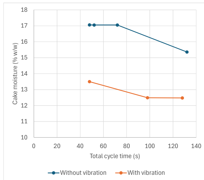
Figure 8 Effect of vibration on cake moisture at varying total cycle times
