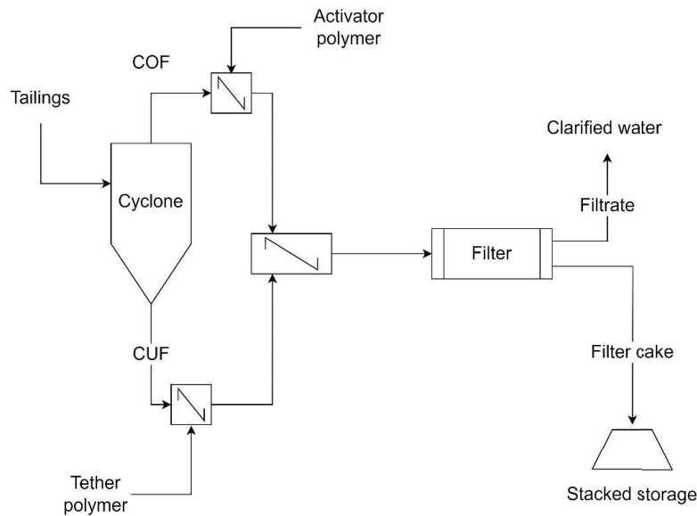
Figure 11 Schematic flow sheet for implementing ATA dewatering
