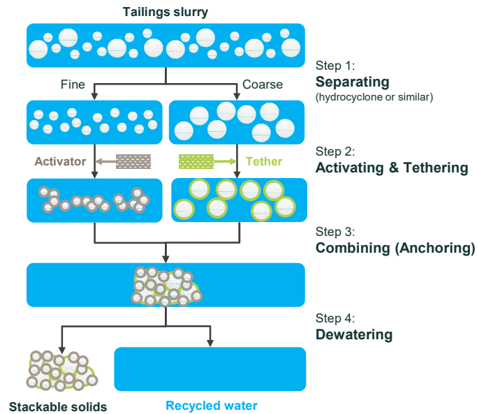
Figure 1 Schematic of the ATA process
